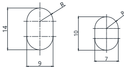
Mounting Hole
